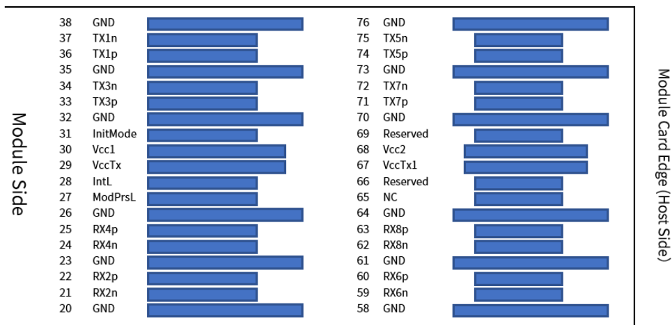
Top side viewed from bottom Legacy QSFP28 Pads Additional QSFP-DD Pads
