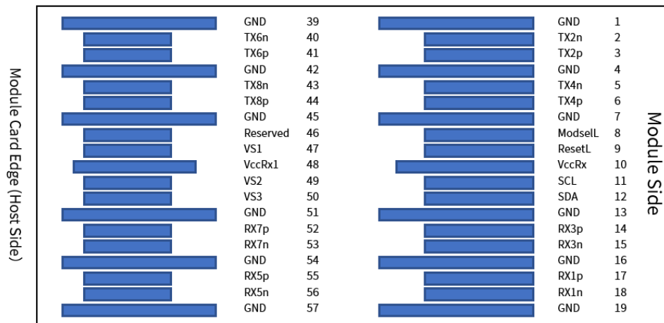
Bottom side viewed from bottom Additional QSFP-DD Pads Legacy QSFP28 Pads
