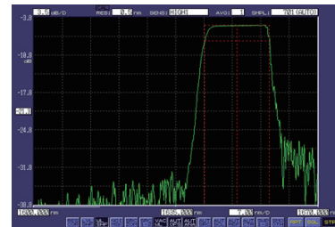
Reflection Spectrum
