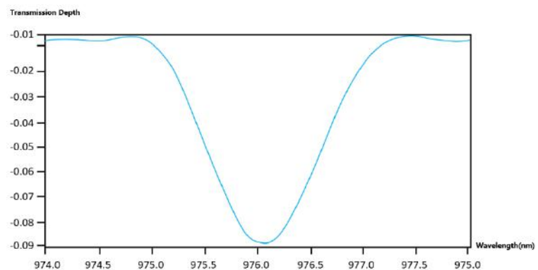
Transmission Spectrum
