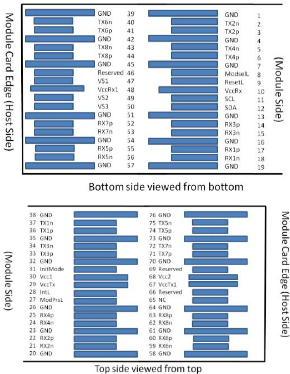
Figure 1 – QSFP-DD -compliant 76-pin connector (per QSFP-DD MSA)
